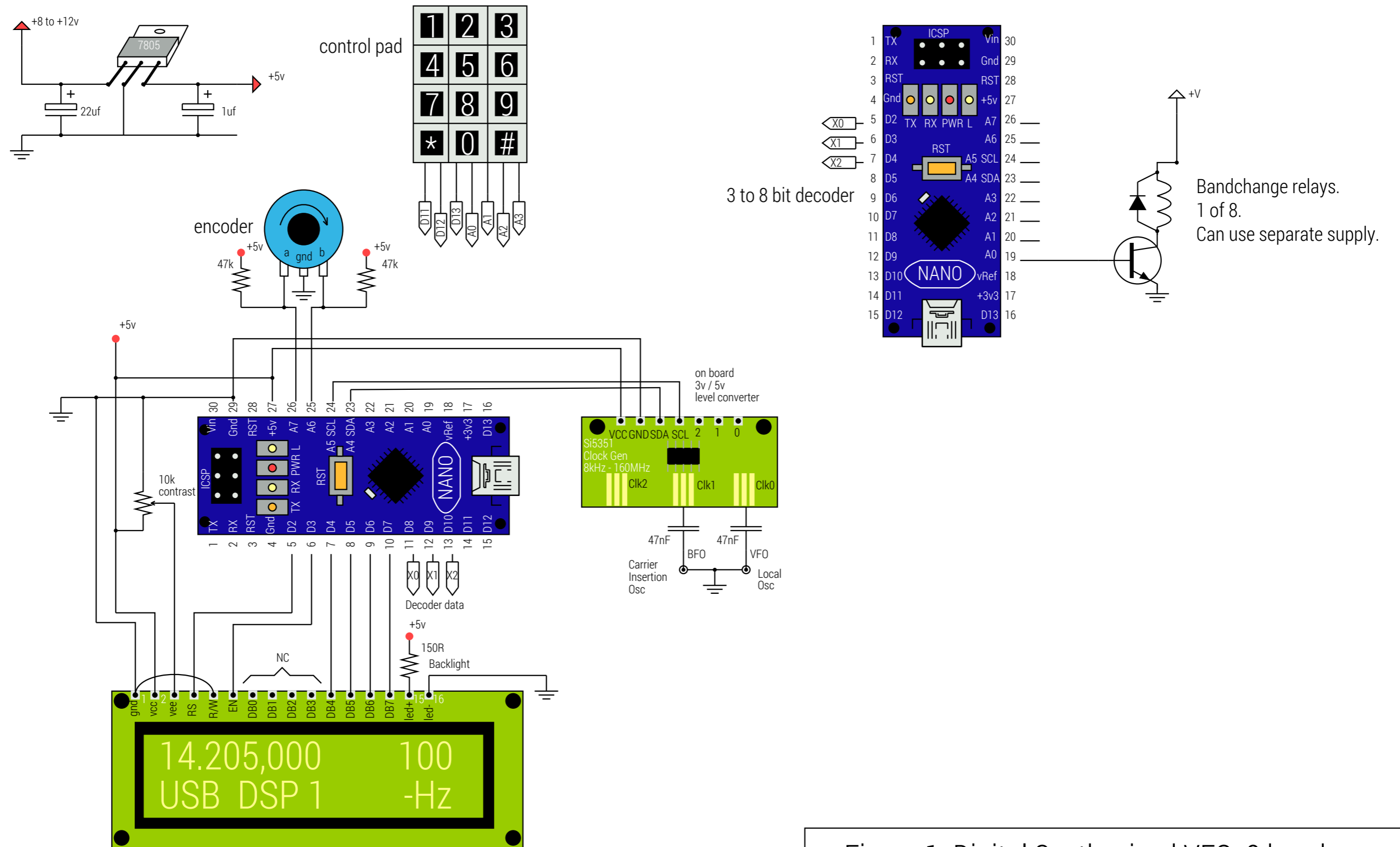
Figure 1. Digital Synthesised VFO. 8 bands
